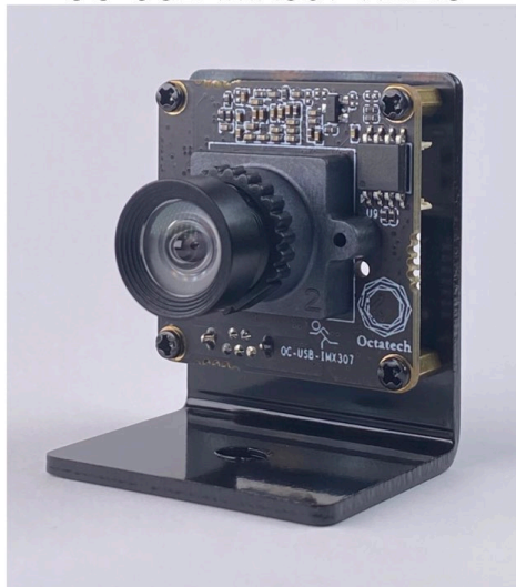
OC-USB-IMX307-ND2.8
